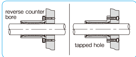
Figure C-14 Examples of Special Installation Hole
