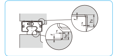
Figure A-58 Mounting Reference Surface Profile
