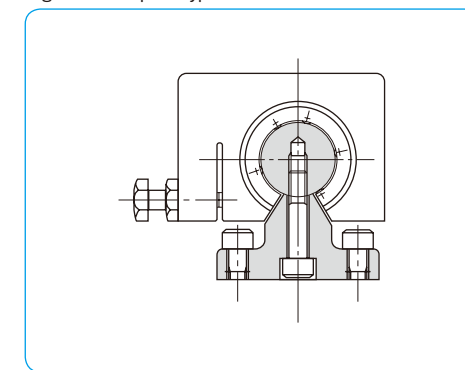
Figure C-6 Open Type
