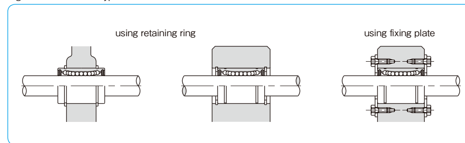
Figure C-5 Clearance Adjustable Type
