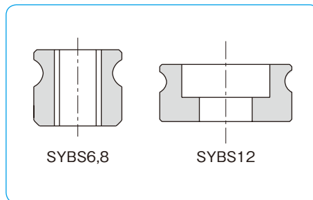
Figure G-25 Profile of SYBS Bed
