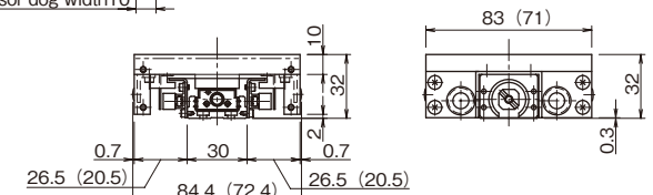
view B (motor bracket A0)
