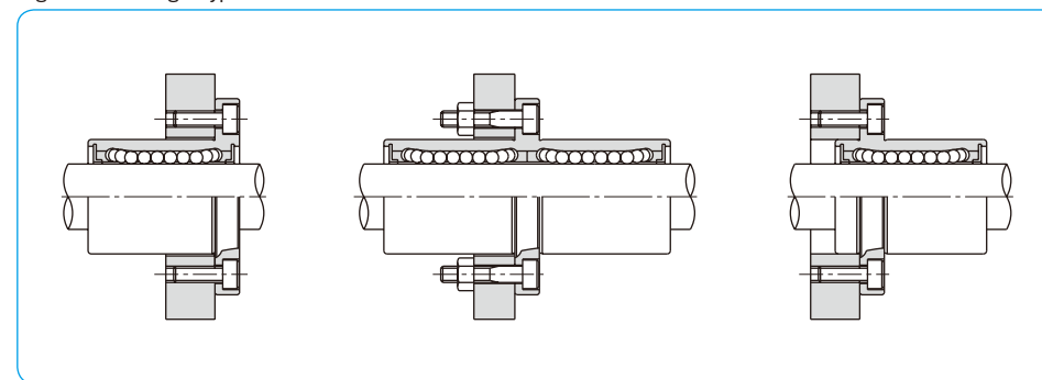
Figure C-7 Flange Type
