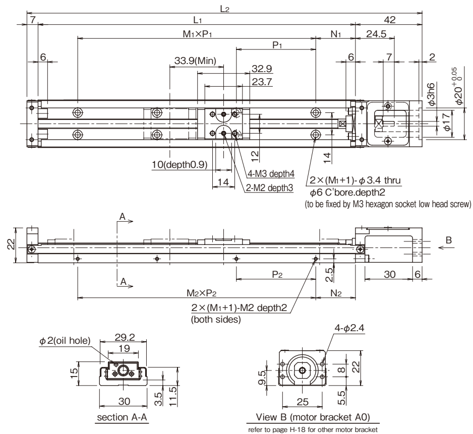
View B (motor bracket A0) refer to page H-18 for other motor bracket
