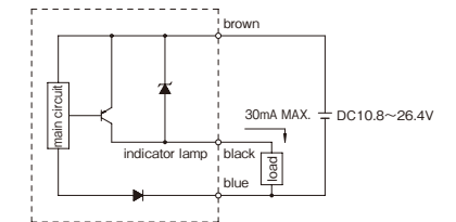
PNP TYPE CIRCUIT DIAGRAM
