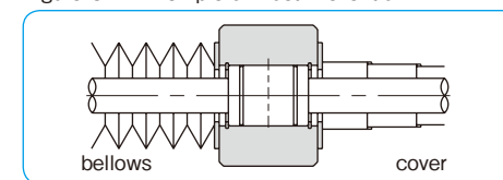
Figure C-12 Example of Dust Prevention
